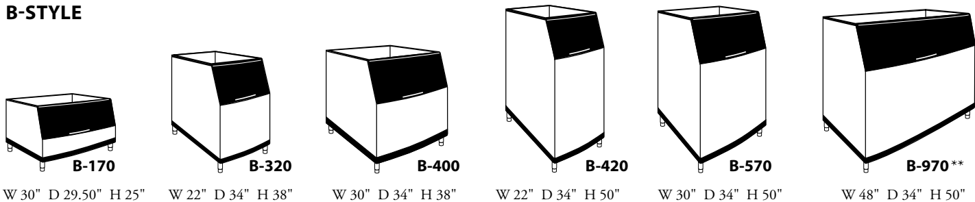
W 30" D 29.50" H 25" W 22" D 34" H 38" W 30" D 34" H 38" W 22" D 34" H 50" W 30" D 34" H 50" W 48" D 34" H 50"
